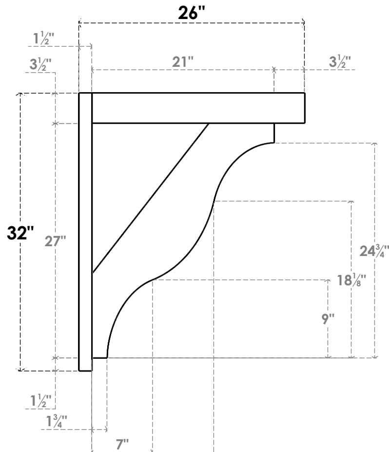
SIDE PROFILE
